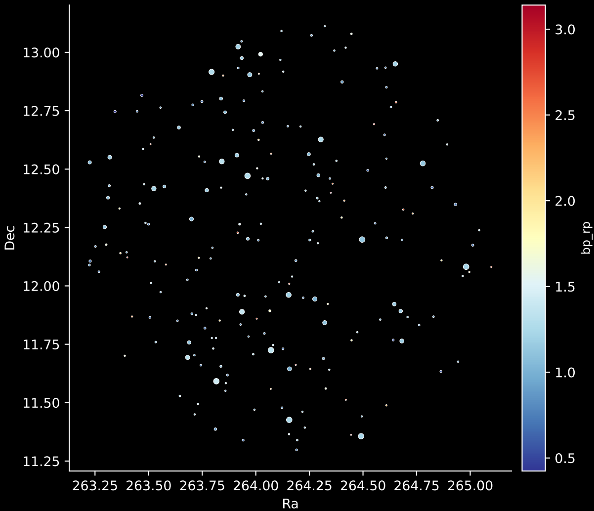
APOGEE DR17 Field: [K2_C14_237+59] Stars: 211
