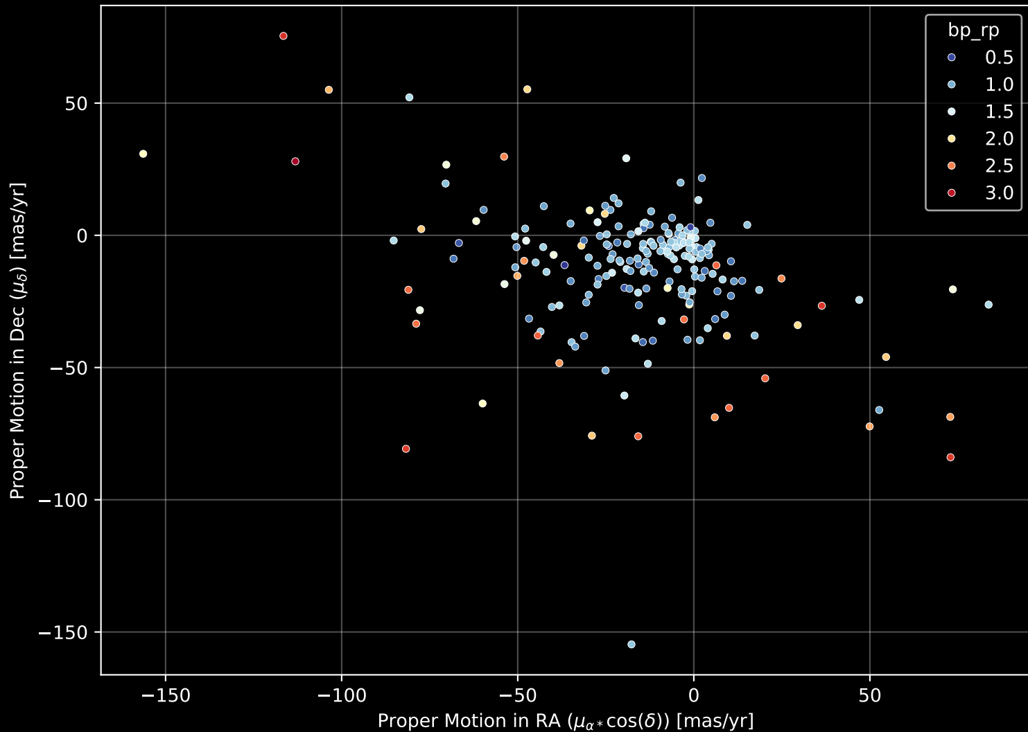
APOGEE DR17 Field: [K2_C14_237+59] Proper Motion Diagram (n= 211)
