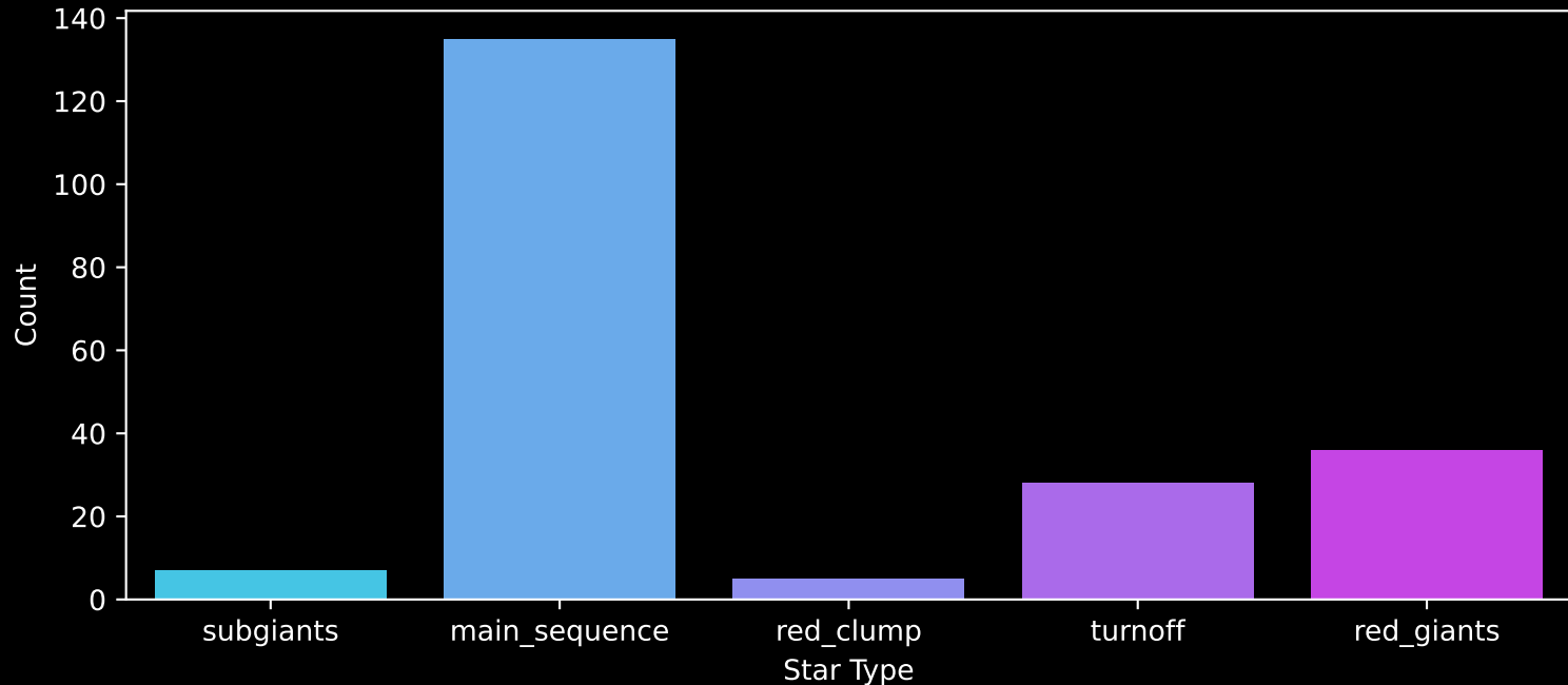
APOGEE DR17 Field: [K2_C14_237+59] Count plot of Star Type
