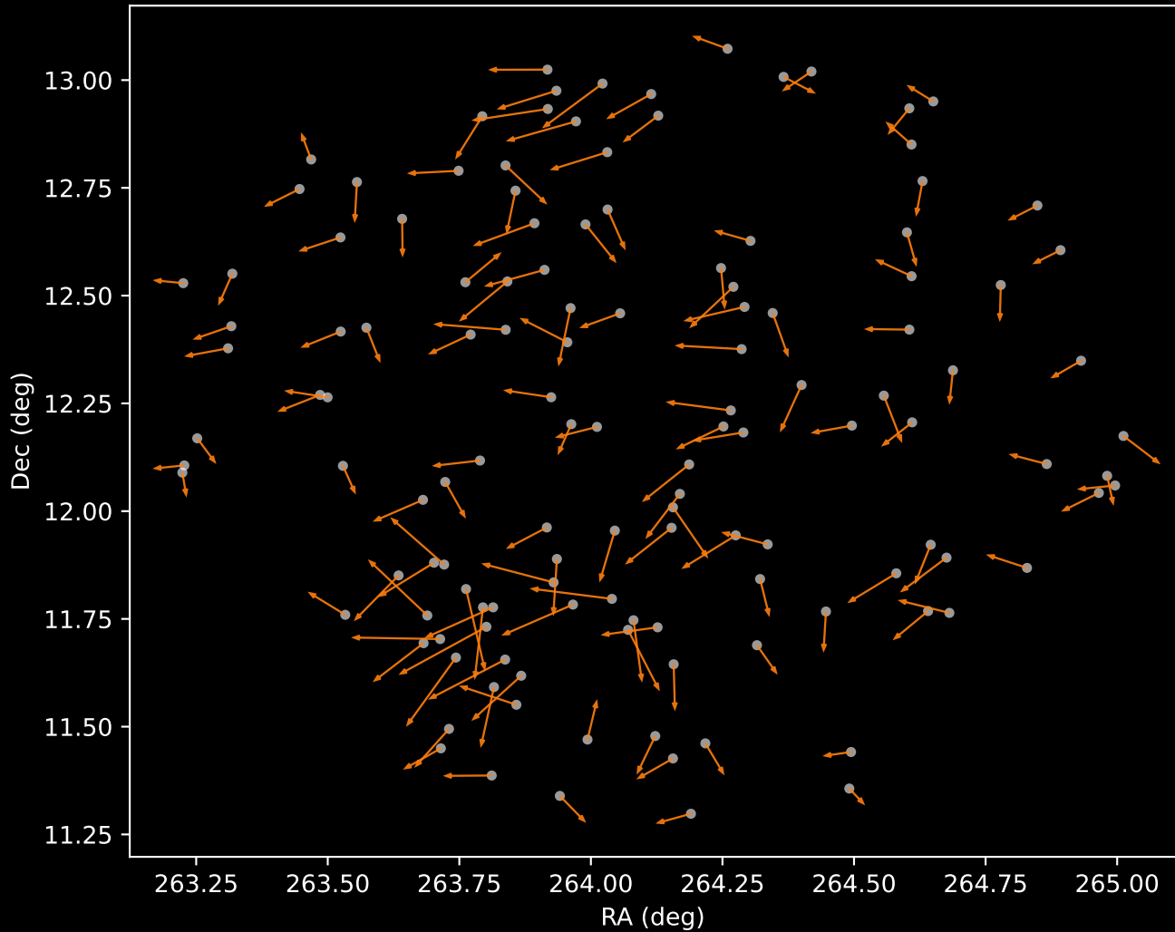
APOGEE DR17 Cluster 2 Proper Motion Vectors (n=131)
