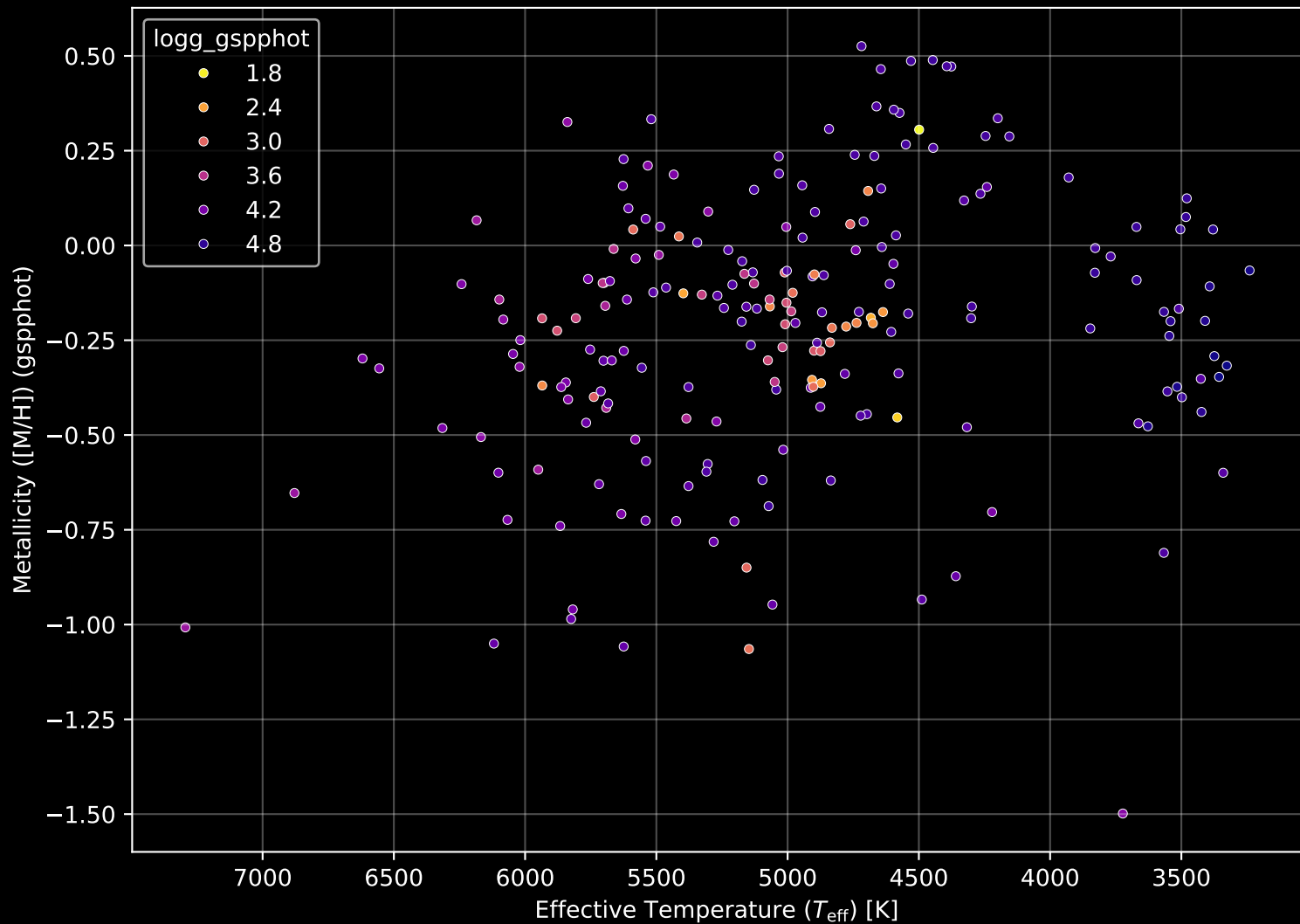
APOGEE DR17 Field: [K2_C14_237+59] Stellar Population Parameters (n= 211)
