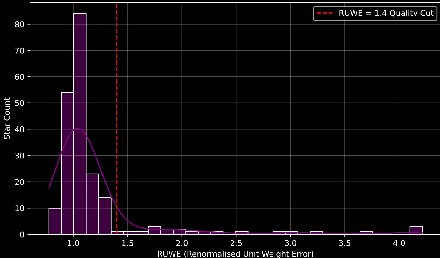
GAPOGEE DR17 Field [K2_C14_237+59] RUWE Distribution (n= 206)
