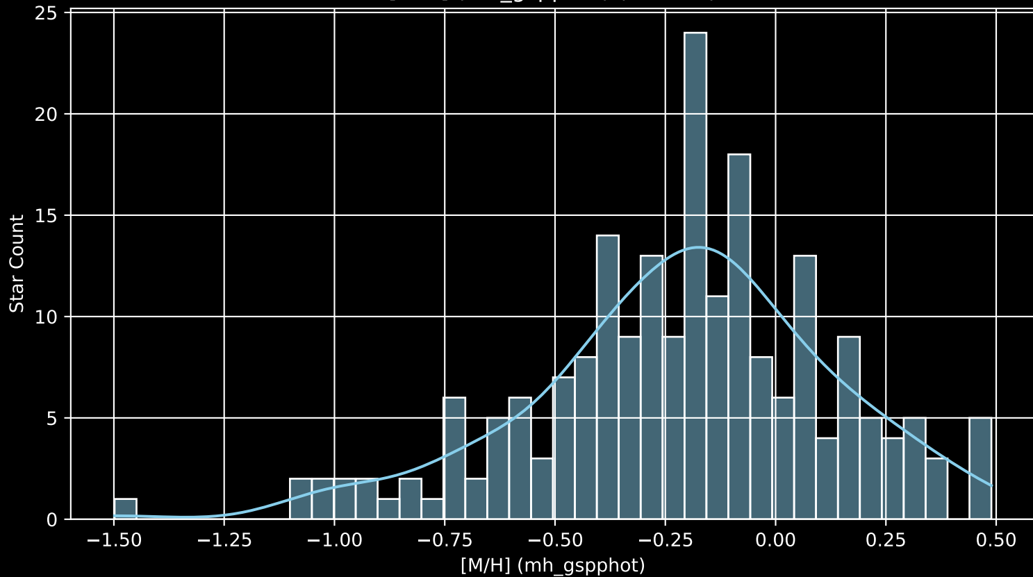
APOGEE DR17 Field: [K2_C14_237+59 [M/H] (mh_gspphot) (n= 210)
