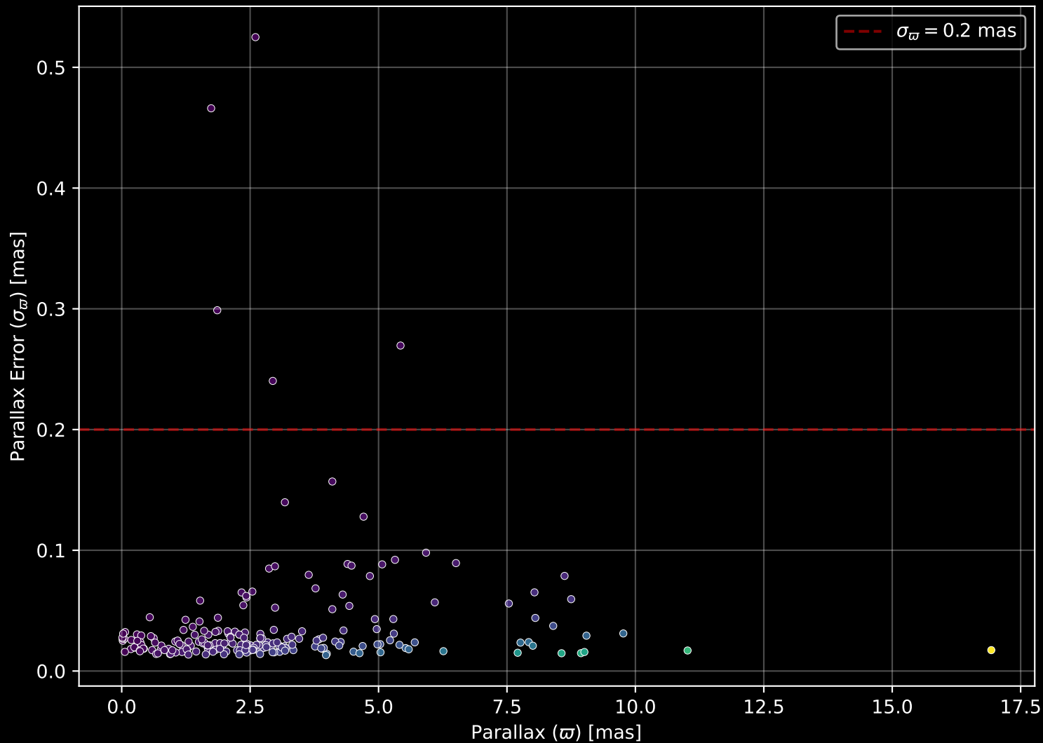
APOGEE DR17 Field: [K2_C14_237+59] Parallax Quality (n= 211)
